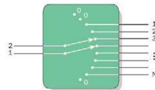
Non-Blocking 2xN
